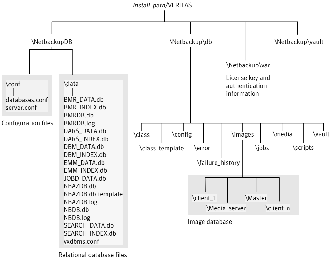
Figure 17-1 Catalog configuration
