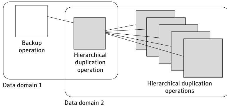
Figure 14-5 Hierarchical operations
