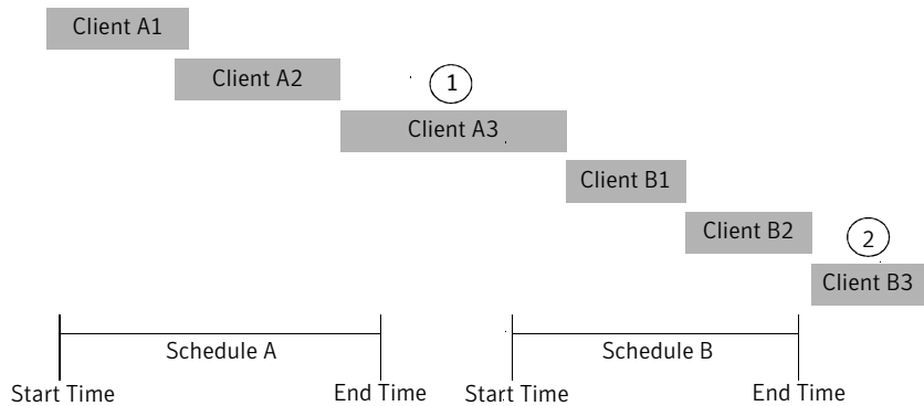
Figure 15-14 Duration example
