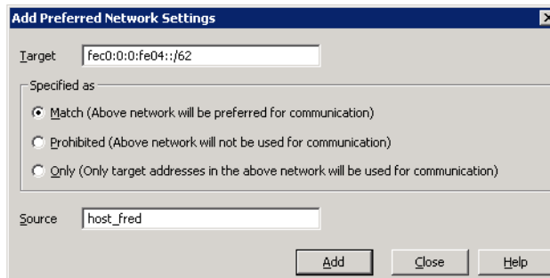
Figure 3-51 Indicating a range of IPv6 networks
