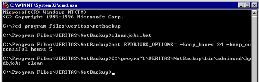
Figure 21-5 Running cleanjobs.bat
