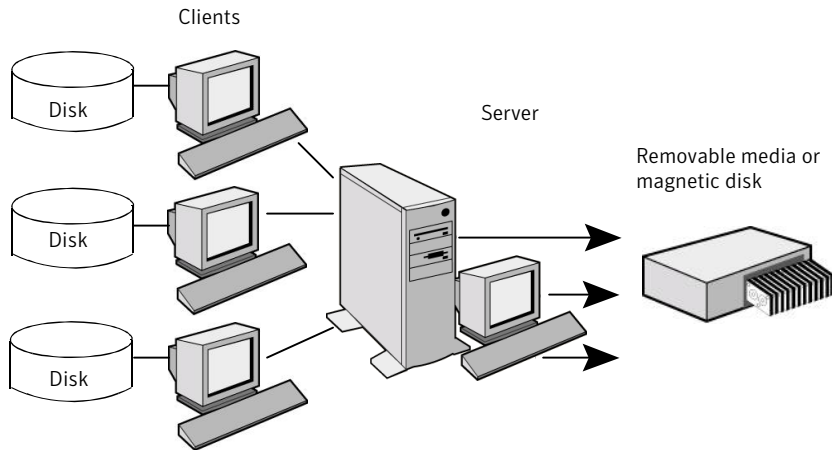
Figure 15-12 Multiplexed backups
