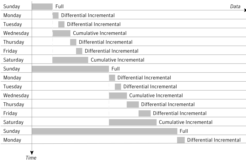
Figure 15-17 Schedule coverage
